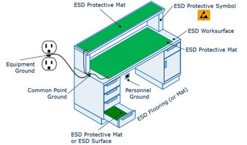
Figure 2: Typical ESD Workstation
